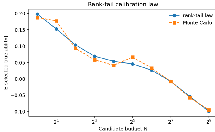
Figure 7: The rank-tail calibration identity matches Monte Carlo selection. Current mean absolute error is 0.0106.
